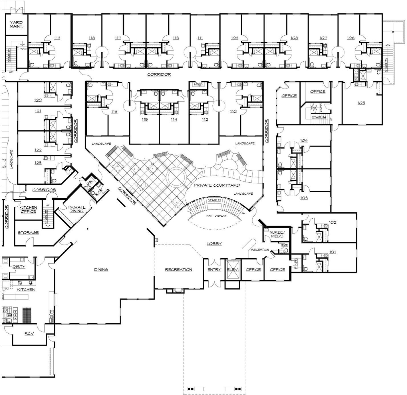
MAIN LEVEL FLOOR PLAN - ASSISTED LIVING
